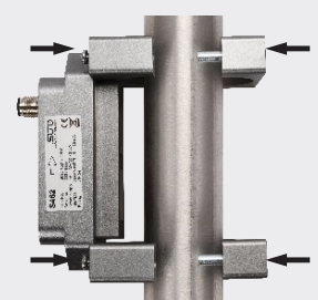
Easy clamp-on installation through mounting brackets
